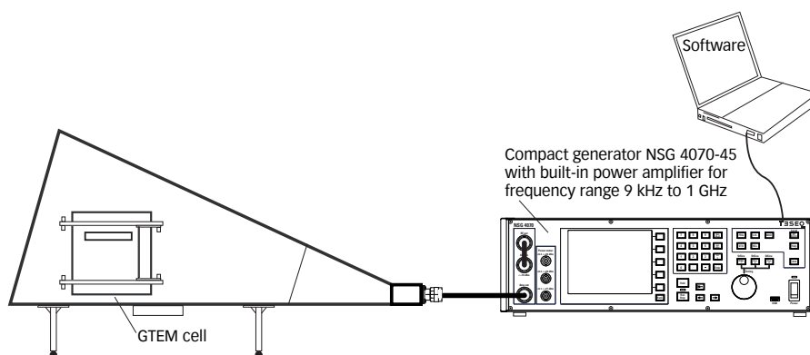
Application for IEC / EN 61000-4-20 up to 1 GHz (example with NSG 4070-45; field probe control requires optional software e.g. WIN 6000)
