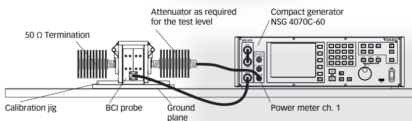
Application for automotive BCI, calibration set-up (example with NSG 4070C-60)
